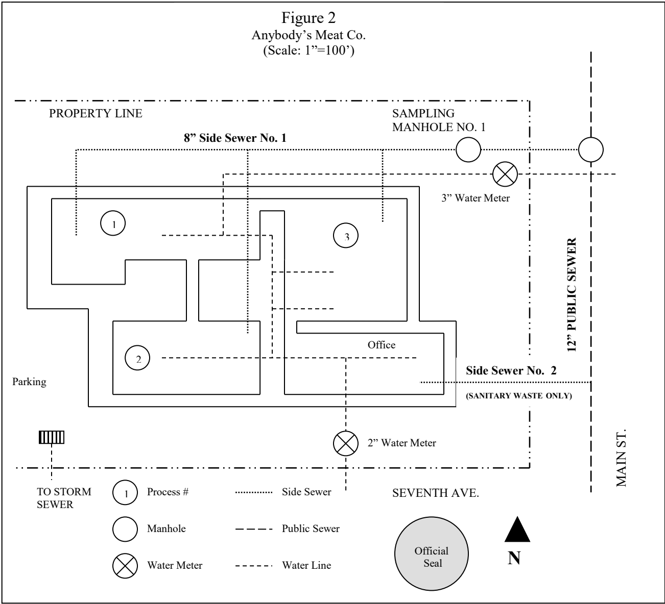
FIGURE 2 - BUILDING LAYOUT
